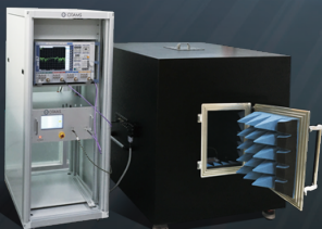
OTA Chamber
