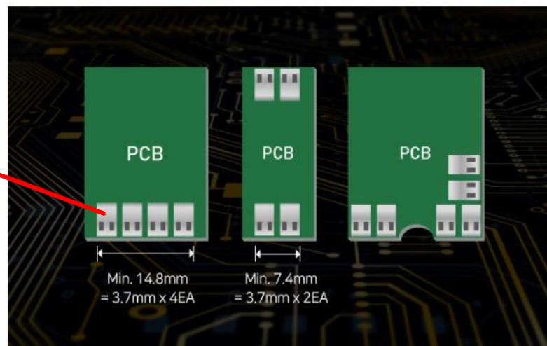
Example _ Antenna modules
