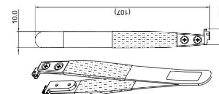
Tweezer for mating and unmating a plug (P/N : GJSZZA1)
